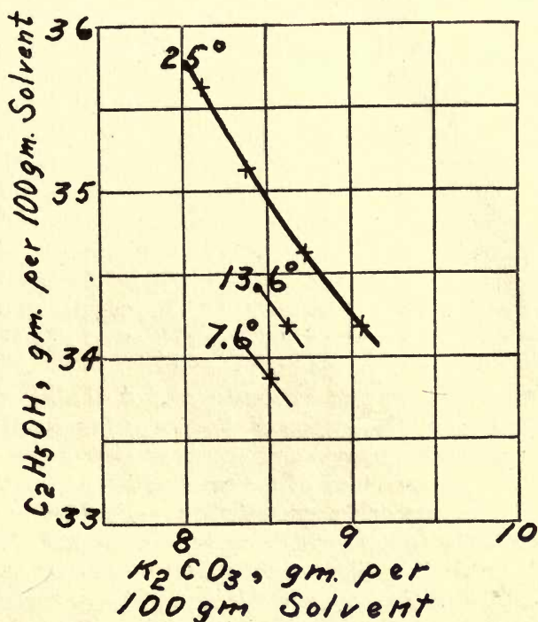
Figure 15. Isotherms in the System: Potassium Carbonate, Ethyl Alcohol, Water.
